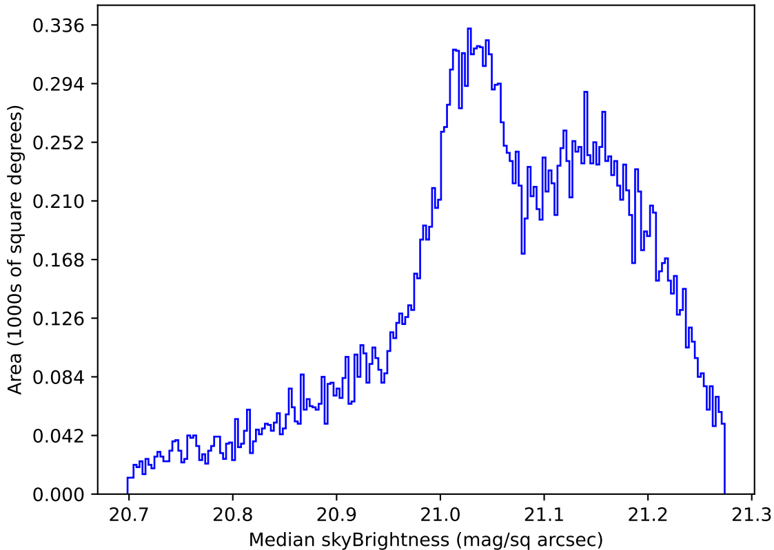
early_u_fpextra3.0_v3.4_10yrs All sky r band: Median skyBrightness
