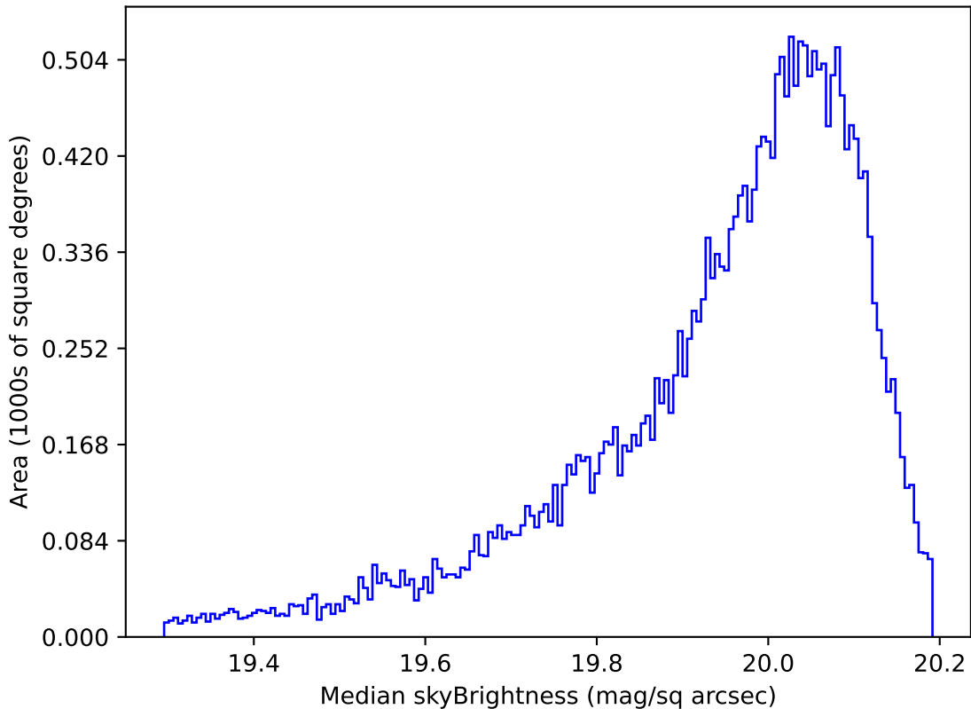
early_u_fpextra3.0_v3.4_10yrs All sky i band: Median skyBrightness
