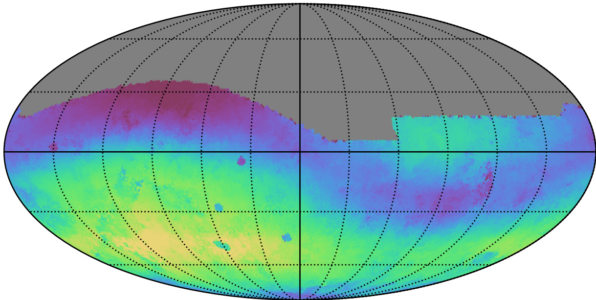
early_u_fpextra3.0_v3.4_10yrs All sky g band: Median skyBrightness
