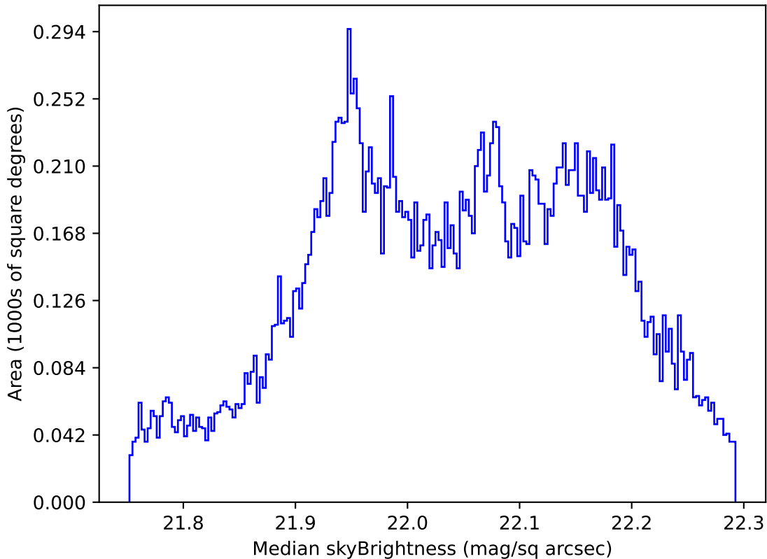
early_u_fpextra3.0_v3.4_10yrs All sky g band: Median skyBrightness
