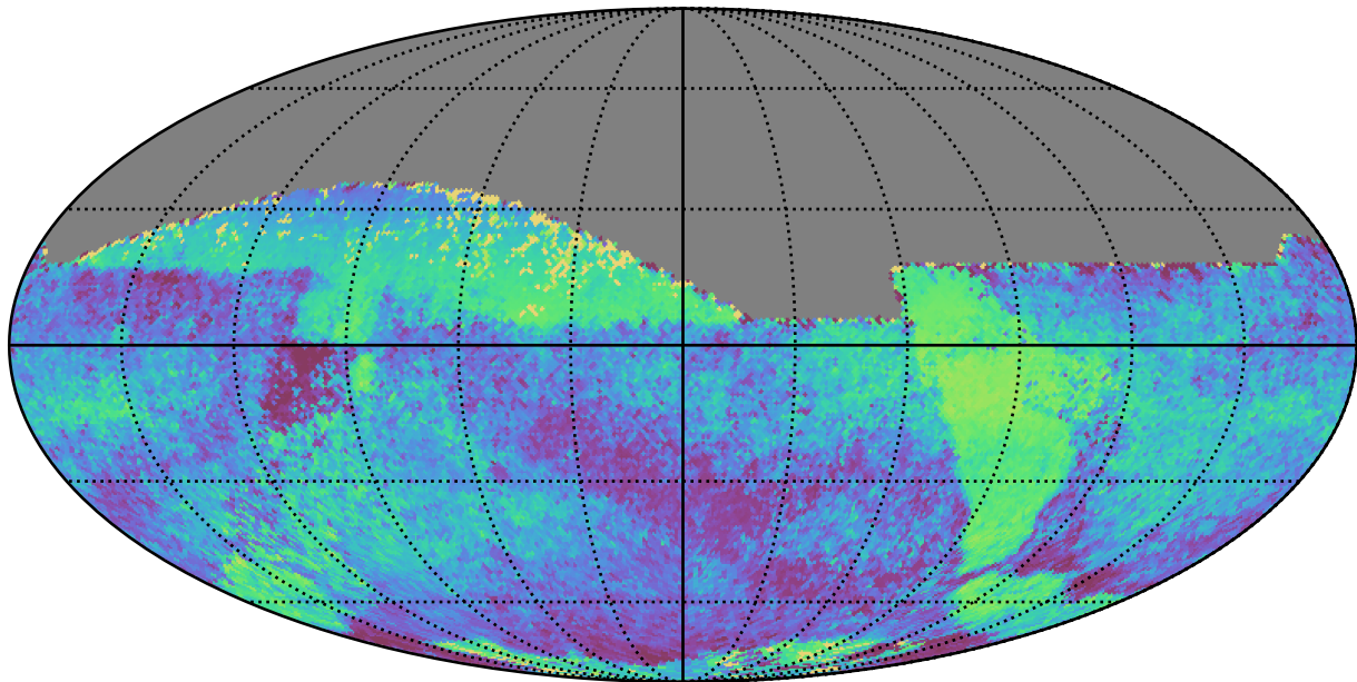
early_u_fpextra3.0_v3.4_10yrs All sky all bands: Median skyBrightness
