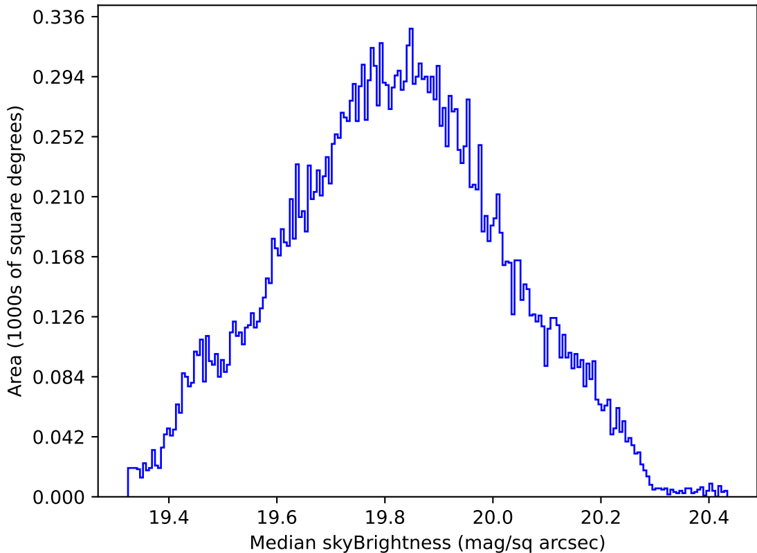
early_u_fpextra3.0_v3.4_10yrs All sky all bands: Median skyBrightness
