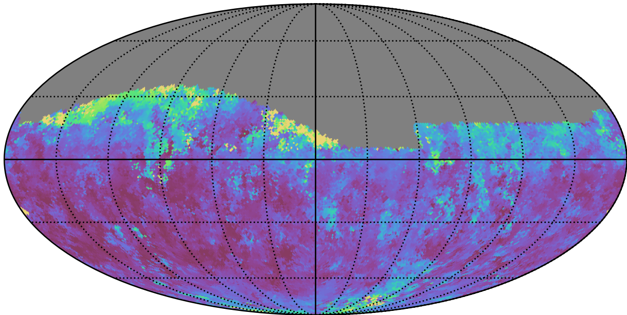
early_u_fpextra3.0_v3.4_10yrs Yr 1 z band: Median seeingGeom
