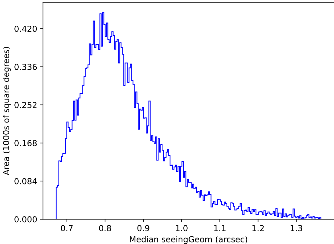
early_u_fpextra3.0_v3.4_10yrs Yr 1 z band: Median seeingGeom
