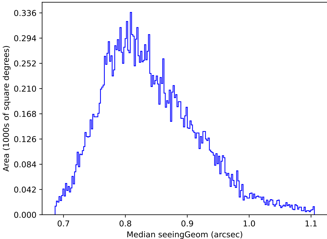
early_u_fpextra3.0_v3.4_10yrs Yr 1 y band: Median seeingGeom
