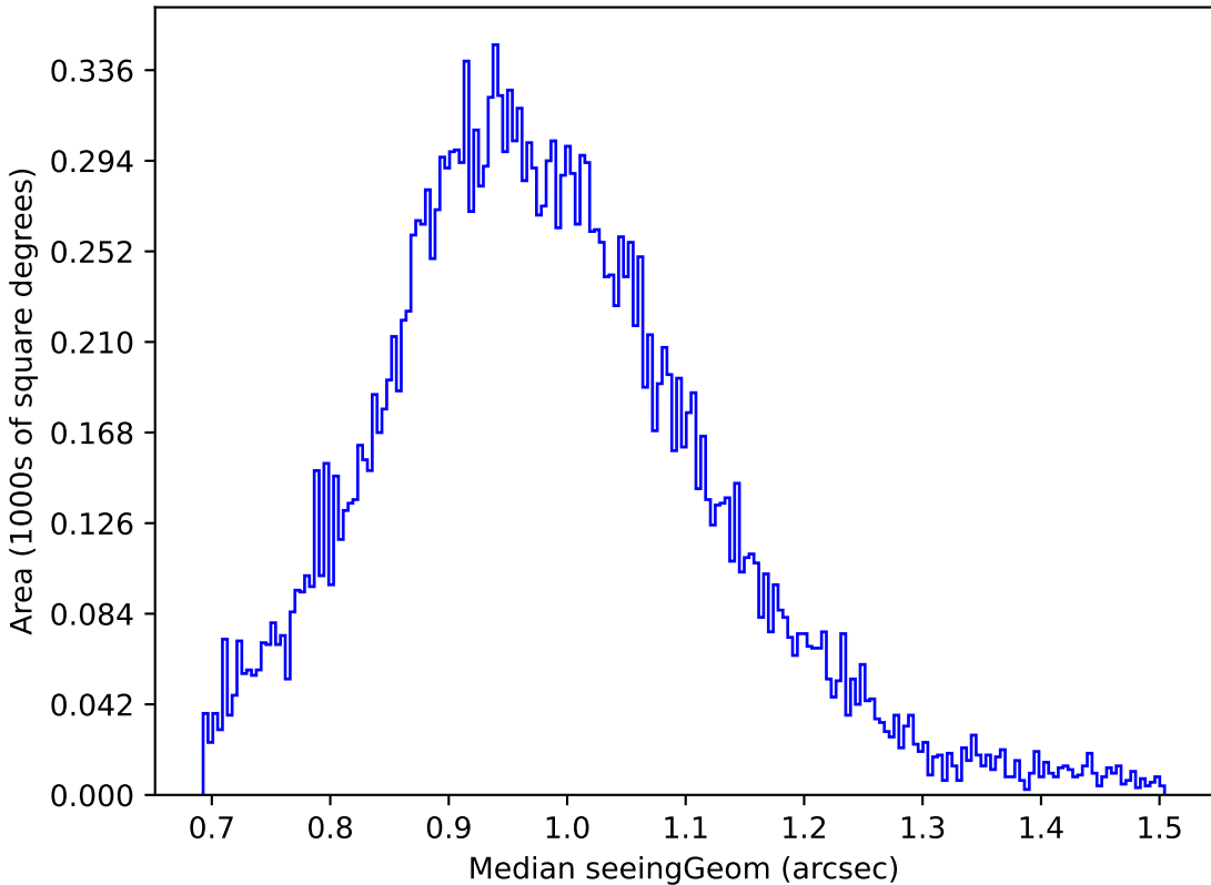
early_u_fpextra3.0_v3.4_10yrs Yr 1 u band: Median seeingGeom
