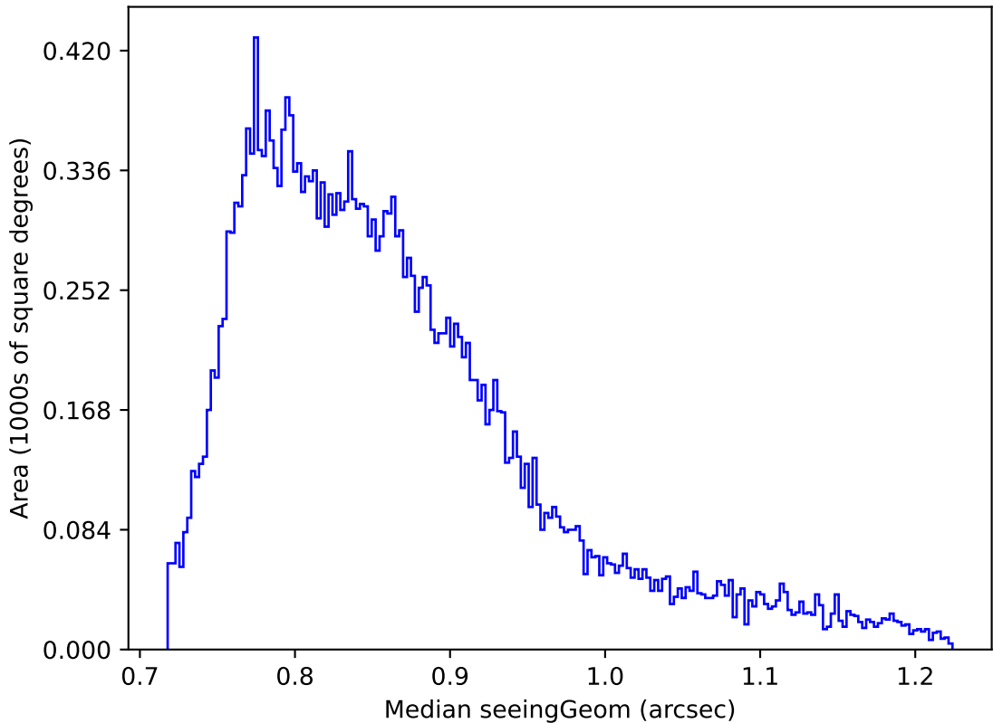
early_u_fpxextra3.0_v3.4_10yrs Yr 1 all bands: Median seeingGeom
