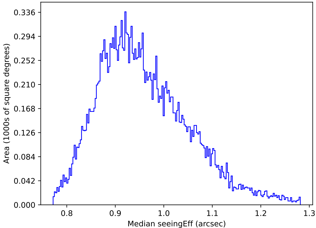
early_u_fpextra3.0_v3.4_10yrs Yr 1 y band: Median seeingEff
