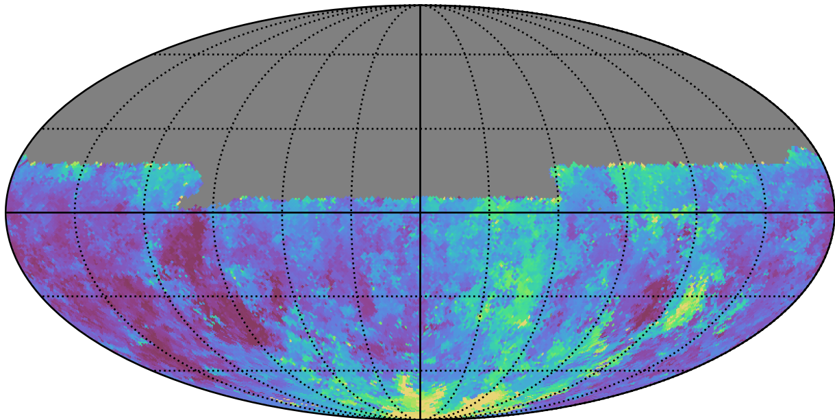
early_u_fpextra3.0_v3.4_10yrs Yr 1 u band: Median seeingEff
