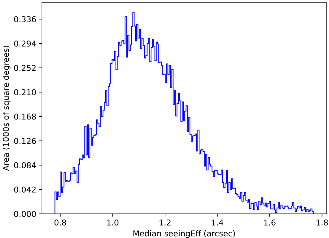
early_u_fpextra3.0_v3.4_10yrs Yr 1 u band: Median seeingEff
