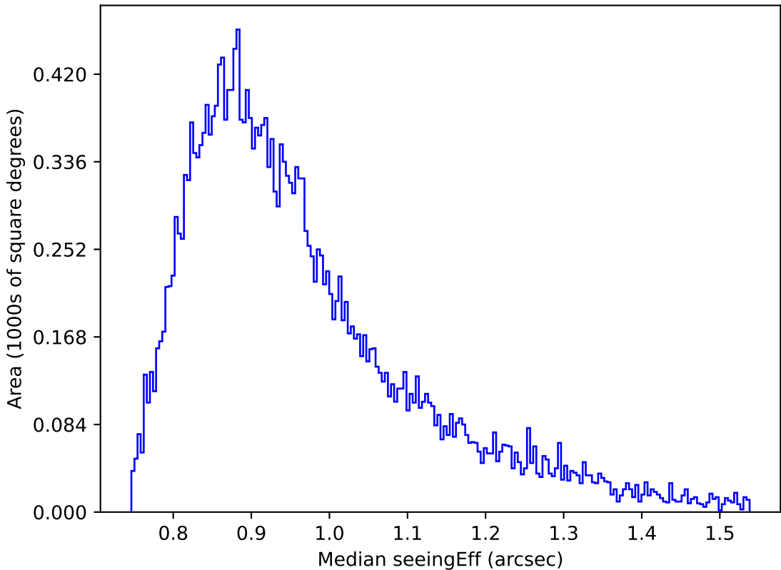
early_u_fpextra3.0_v3.4_10yrs Yr 1 r band: Median seeingEff
