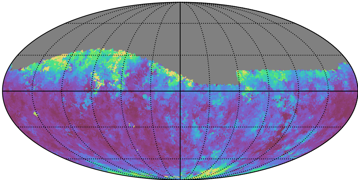
early_u_fpextra3.0_v3.4_10yrs Yr 1 i band: Median seeingEff
