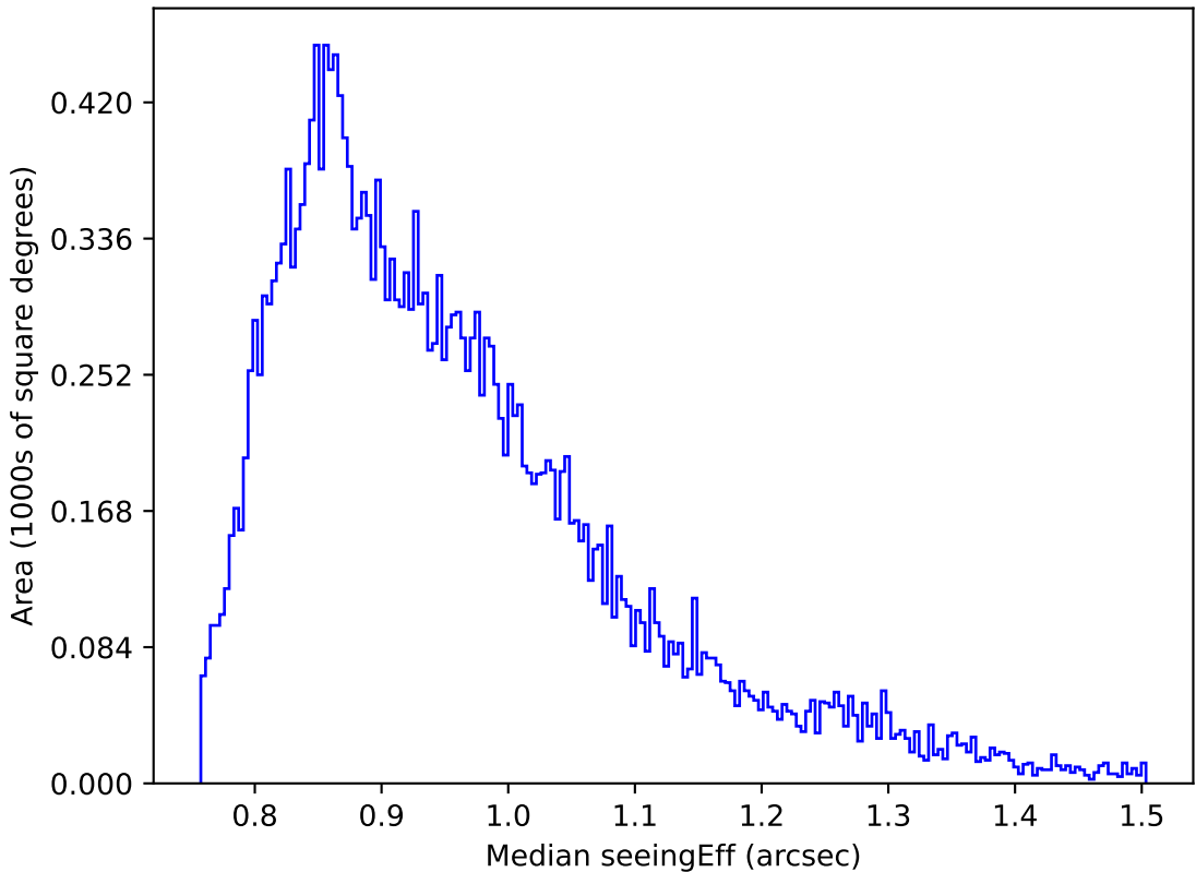
early_u_fpextra3.0_v3.4_10yrs Yr 1 i band: Median seeingEff
