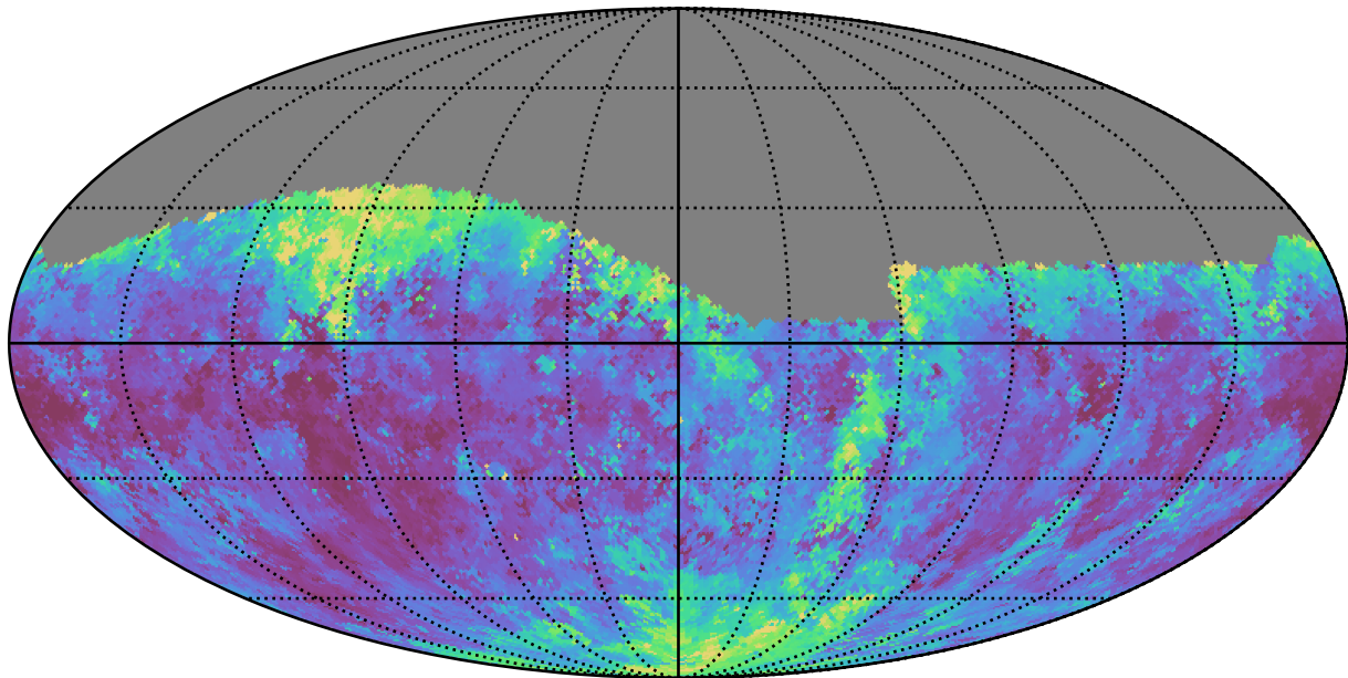
early_u_fpextra3.0_v3.4_10yrs Yr 1 g band: Median seeingEff
