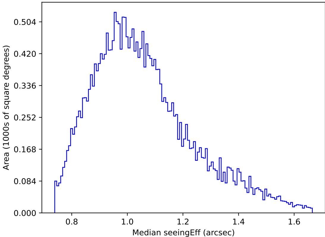
early_u_fpextra3.0_v3.4_10yrs Yr 1 g band: Median seeingEff
