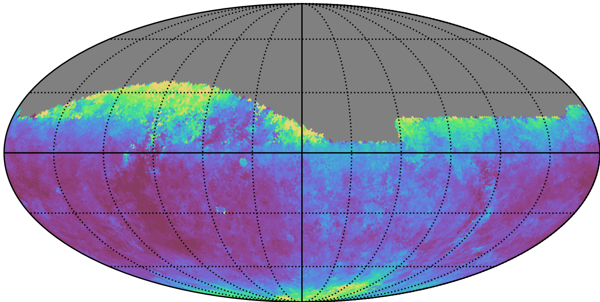
early_u_fpextra3.0_v3.4_10yrs Yr 1 all bands: Median seeingEff
