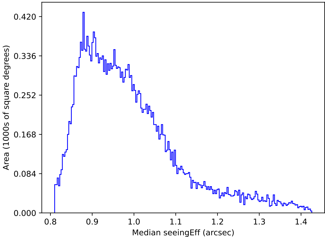
early_u_fpextra3.0_v3.4_10yrs Yr 1 all bands: Median seeingEff
