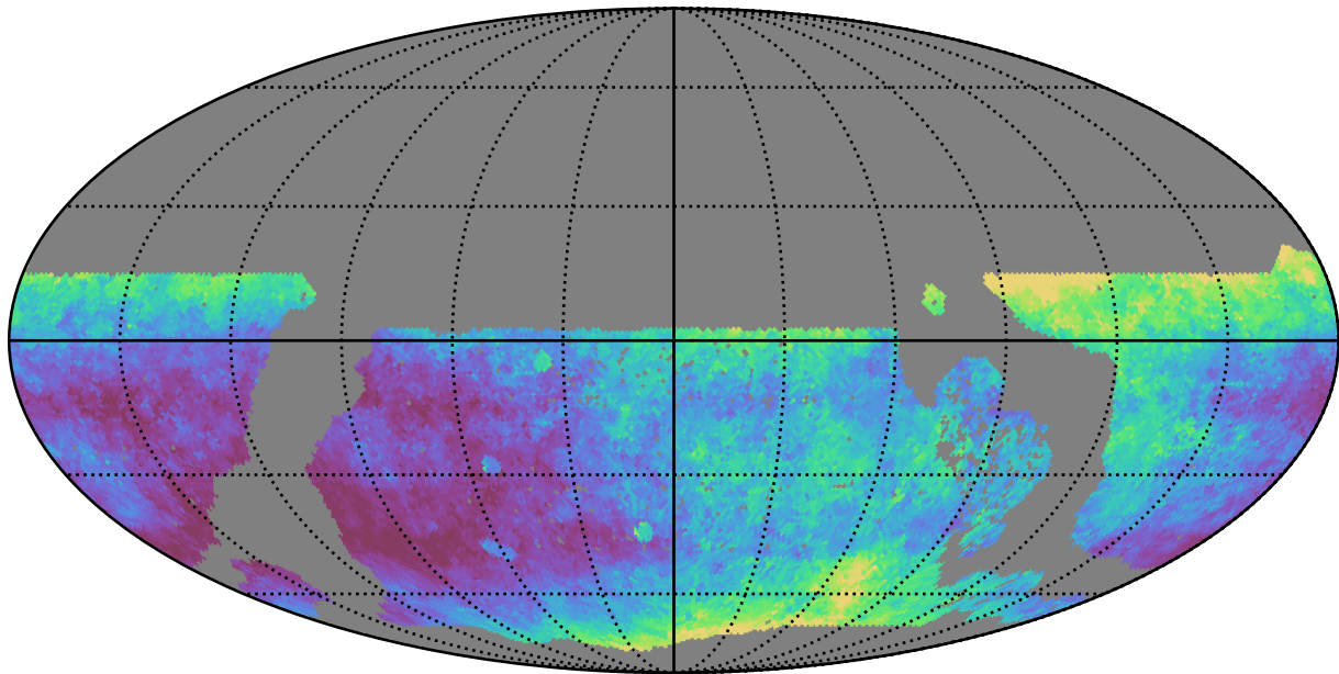
early_u_fpextra3.0_v3.4_10yrs WFD z band: Median seeingEff
