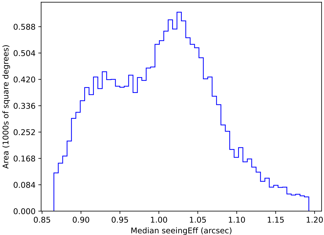
early_u_fpextra3.0_v3.4_10yrs WFD z band: Median seeingEff
