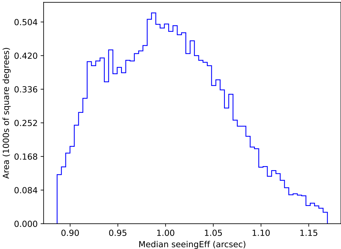
early_u_fpextra3.0_v3.4_10yrs WFD y band: Median seeingEff
