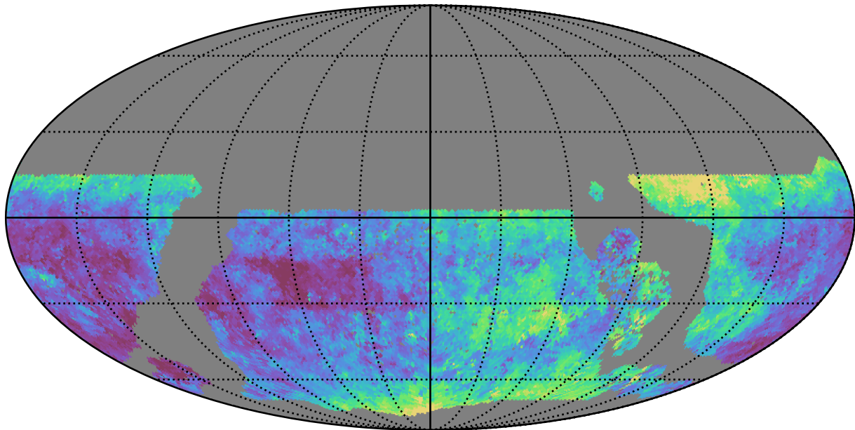
early_u_fpextra3.0_v3.4_10yrs WFD u band: Median seeingEff
