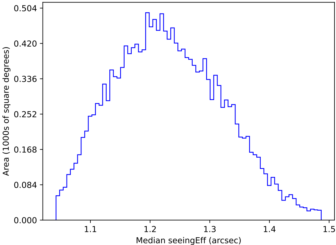
early_u_fpextra3.0_v3.4_10yrs WFD u band: Median seeingEff
