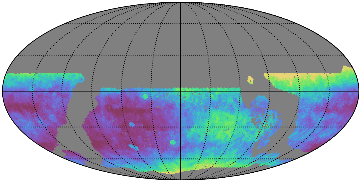
early_u_fpextra3.0_v3.4_10yrs WFD r band: Median seeingEff
