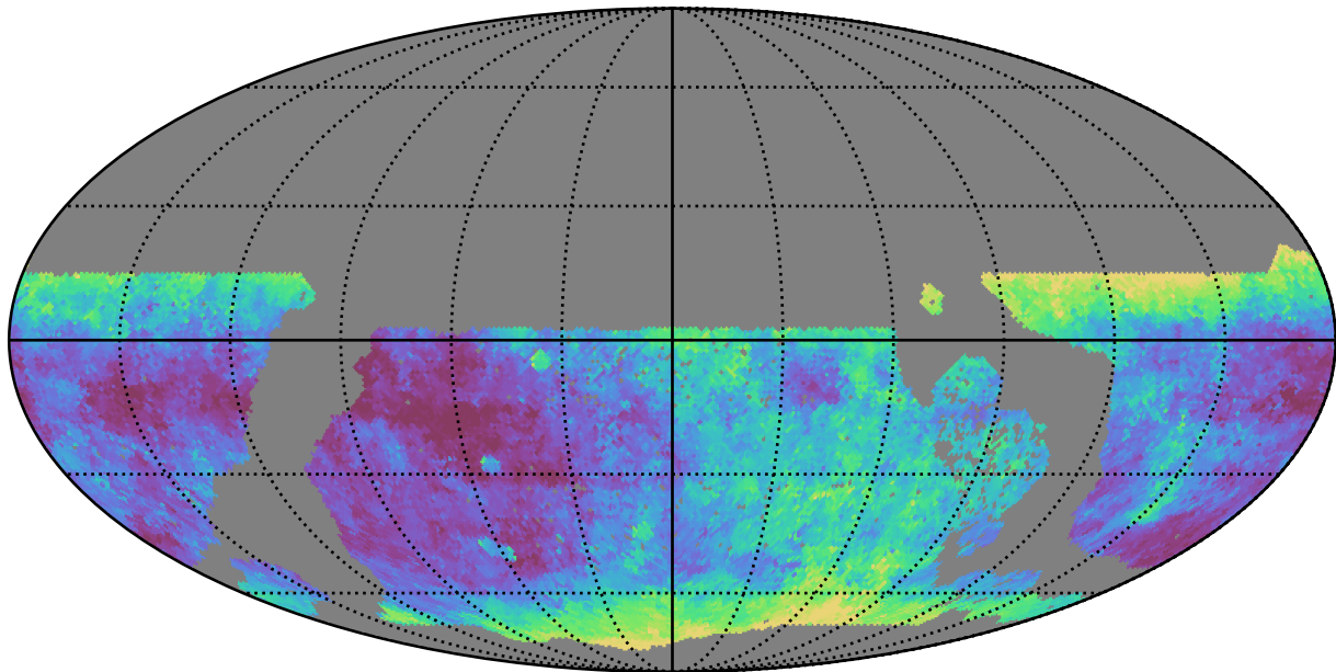
early_u_fpextra3.0_v3.4_10yrs WFD g band: Median seeingEff
