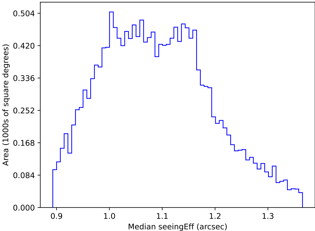
early_u_fpextra3.0_v3.4_10yrs WFD g band: Median seeingEff
