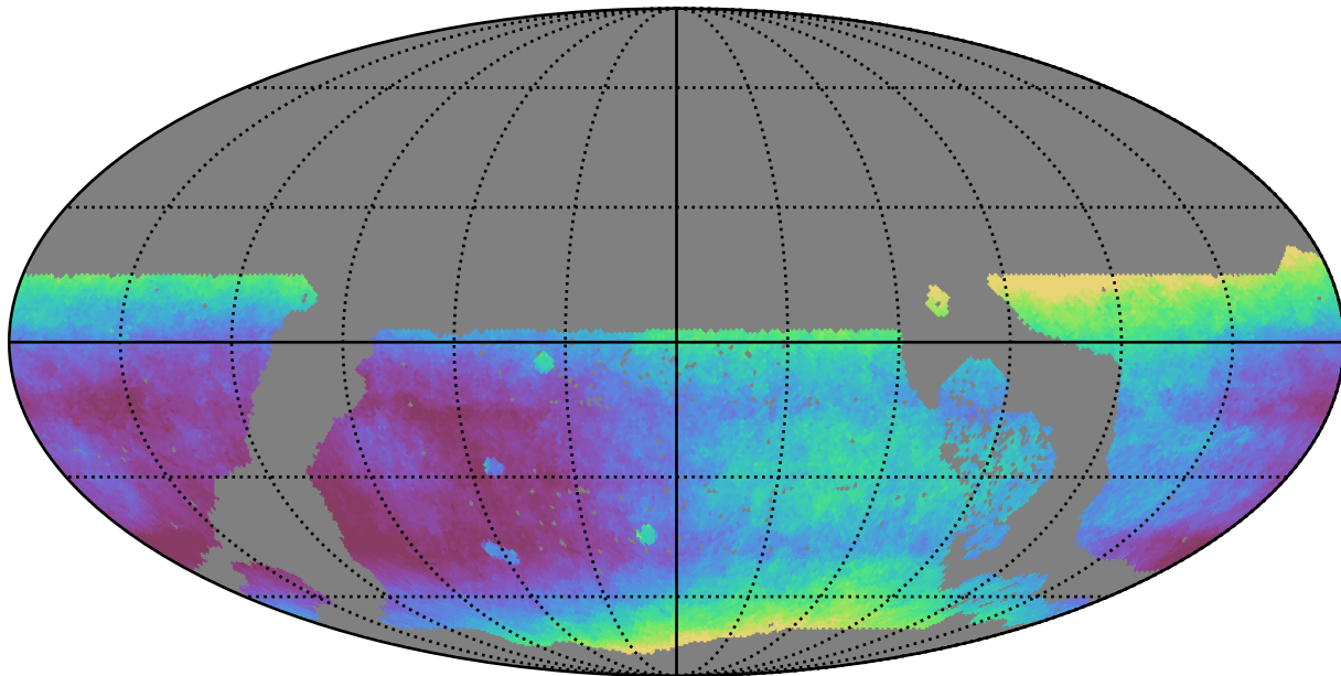
early_u_fpextra3.0_v3.4_10yrs WFD all bands: Median seeingEff
