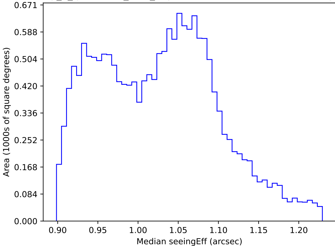
early_u_fpextra3.0_v3.4_10yrs WFD all bands: Median seeingEff
