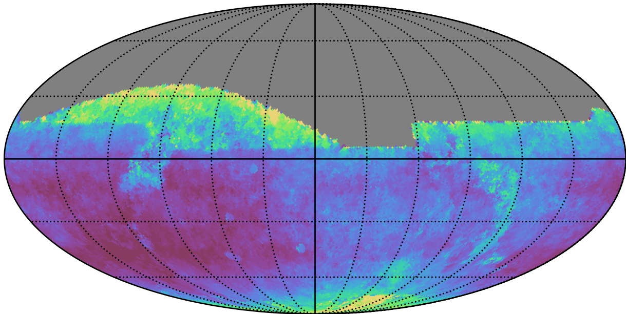
early_u_fpextra3.0_v3.4_10yrs All sky z band: Median seeingEff
