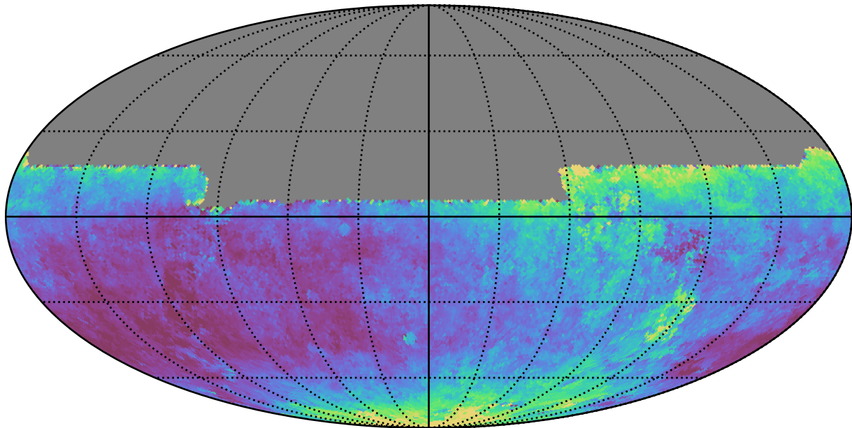
early_u_fpextra3.0_v3.4_10yrs All sky y band: Median seeingEff
