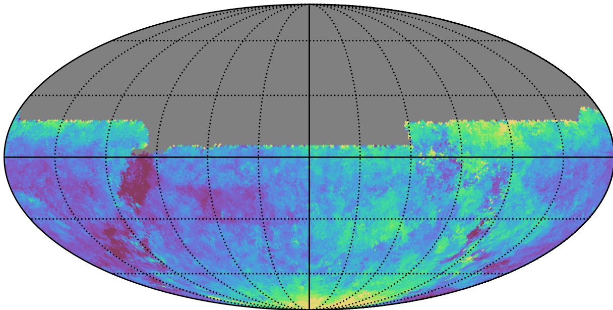
early_u_fpextra3.0_v3.4_10yrs All sky u band: Median seeingEff
