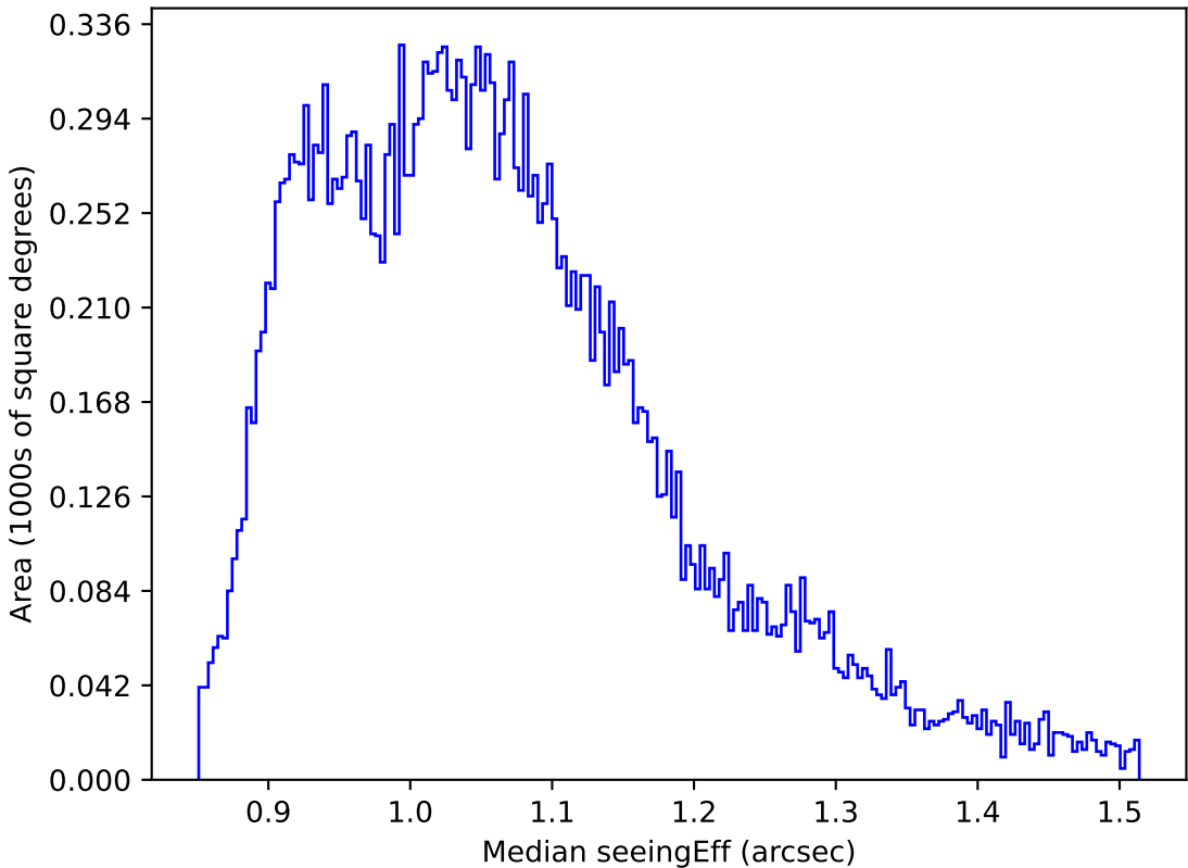
early_u_fpextra3.0_v3.4_10yrs All sky r band: Median seeingEff
