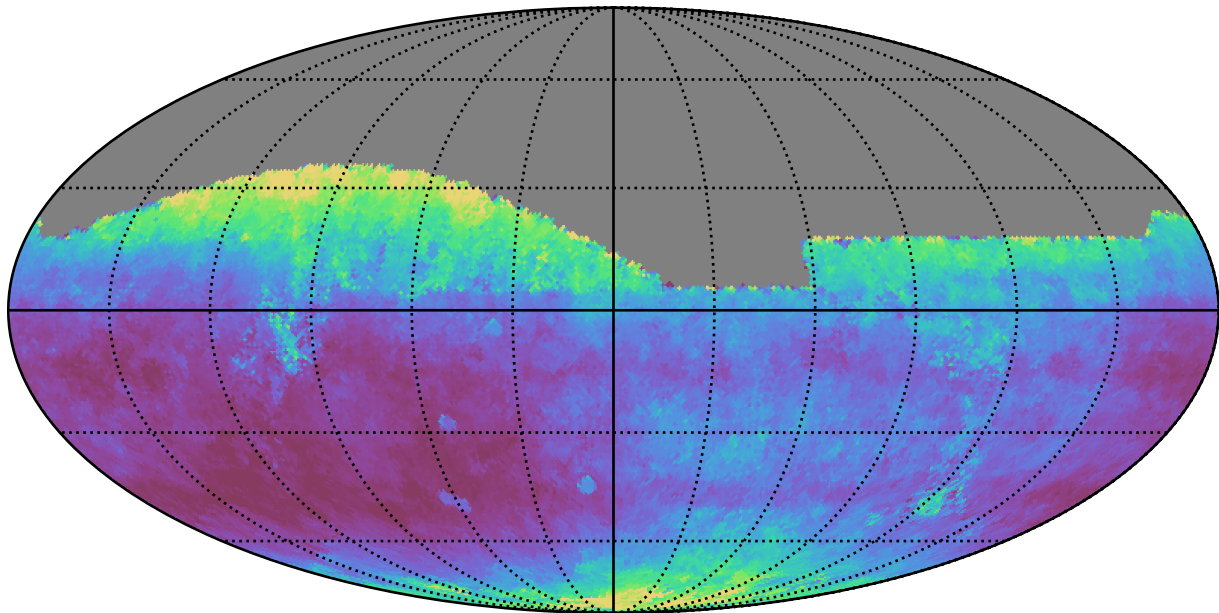
early_u_fpextra3.0_v3.4_10yrs All sky i band: Median seeingEff
