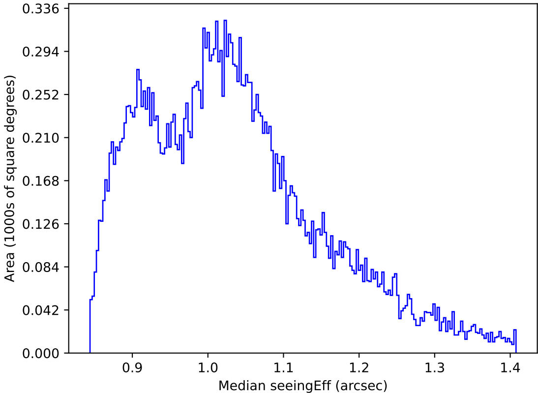
early_u_fpextra3.0_v3.4_10yrs All sky i band: Median seeingEff
