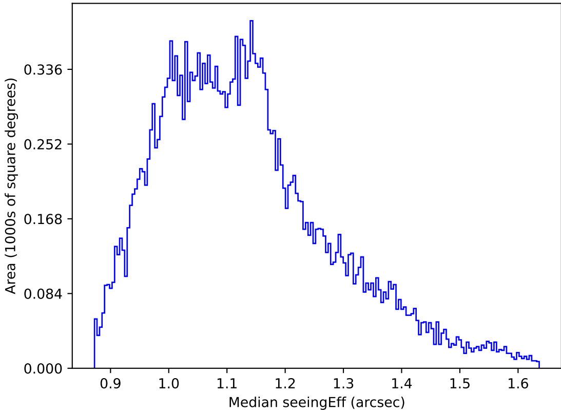
early_u_fpextra3.0_v3.4_10yrs All sky g band: Median seeingEff
