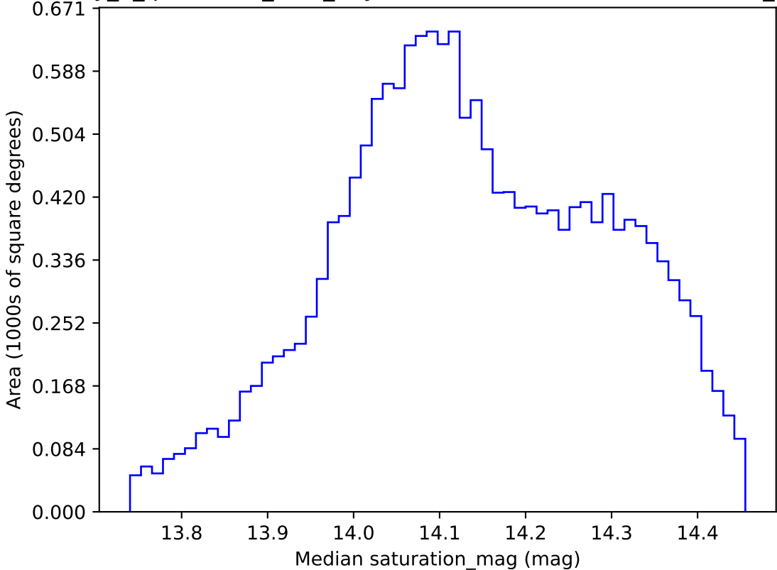
early_u_fpextra3.0_v3.4_10yrs WFD z band: Median saturation_mag
