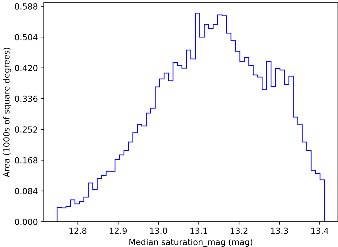
early_u_fpextra3.0_v3.4_10yrs WFD y band: Median saturation_mag
