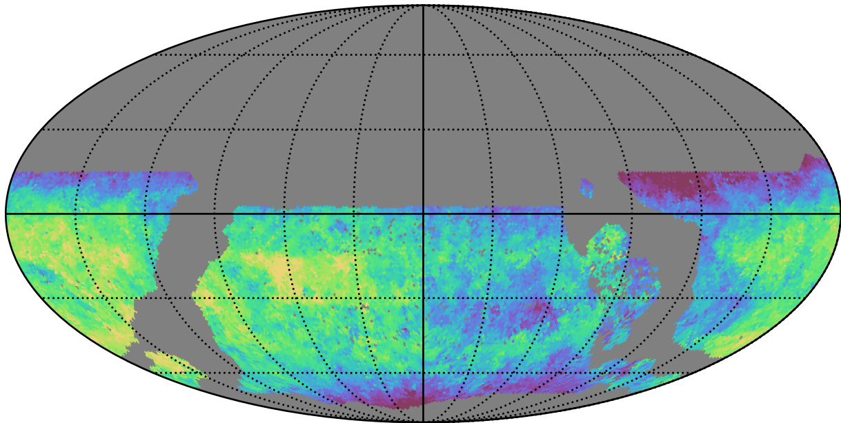
early_u_fpextra3.0_v3.4_10yrs WFD u band: Median saturation_mag
