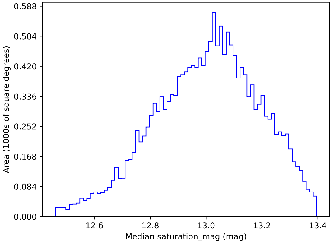
early_u_fpextra3.0_v3.4_10yrs WFD u band: Median saturation_mag
