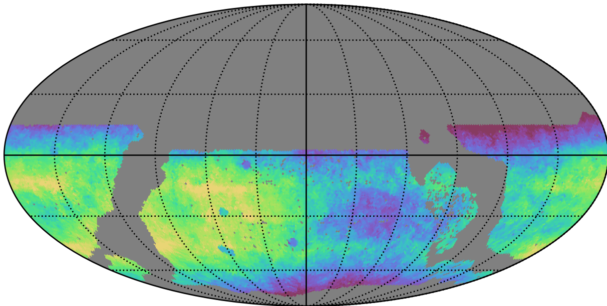
early_u_fpextra3.0_v3.4_10yrs WFD r band: Median saturation_mag
