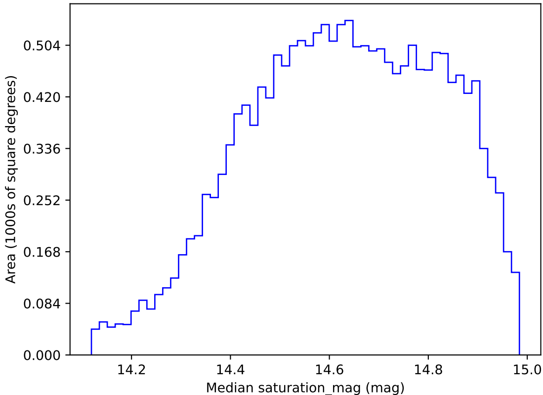
early_u_fpextra3.0_v3.4_10yrs WFD r band: Median saturation_mag
