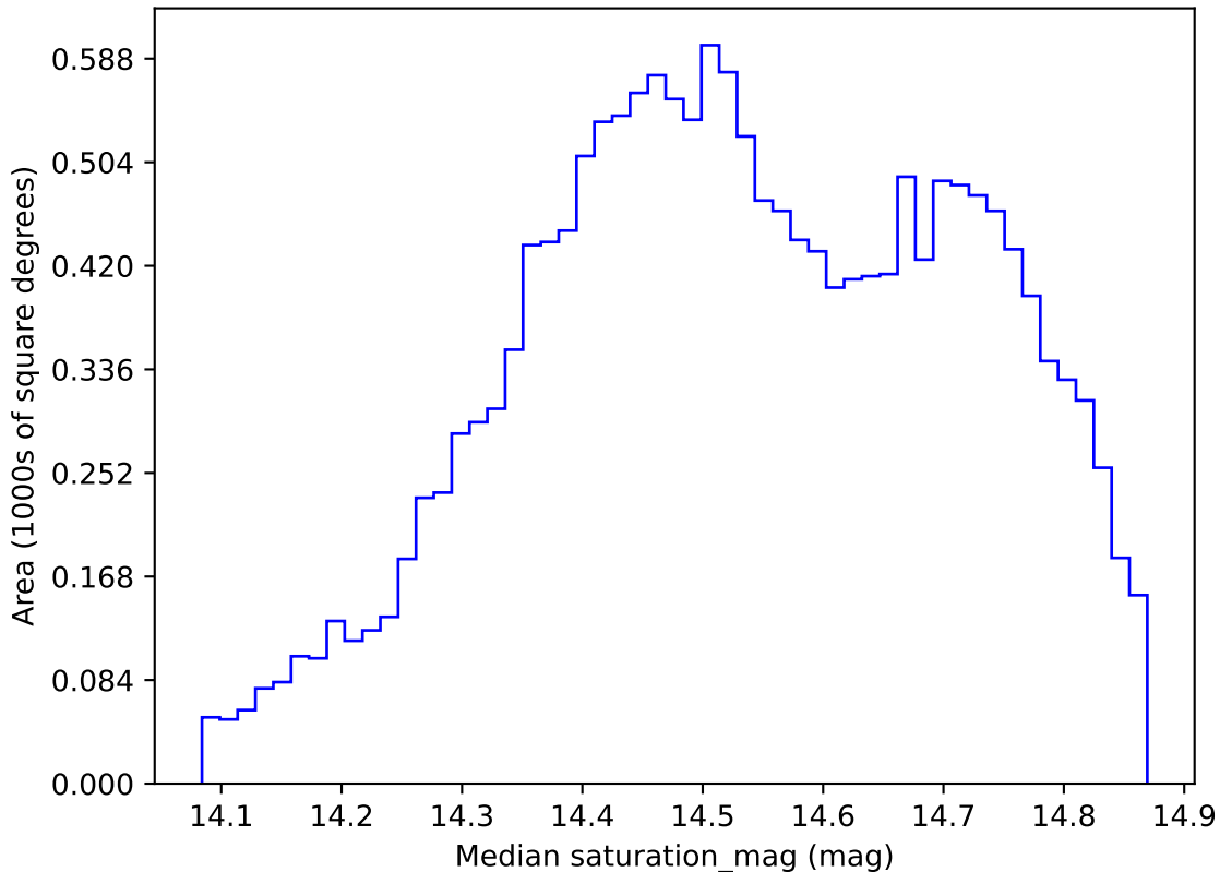
early_u_fpextra3.0_v3.4_10yrs WFD i band: Median saturation_mag
