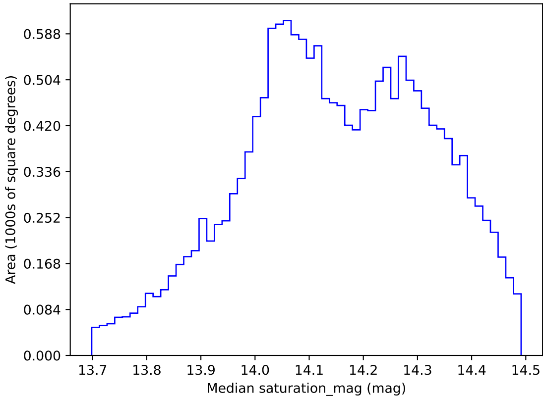
early_u_fpextra3.0_v3.4_10yrs WFD all bands: Median saturation_mag
