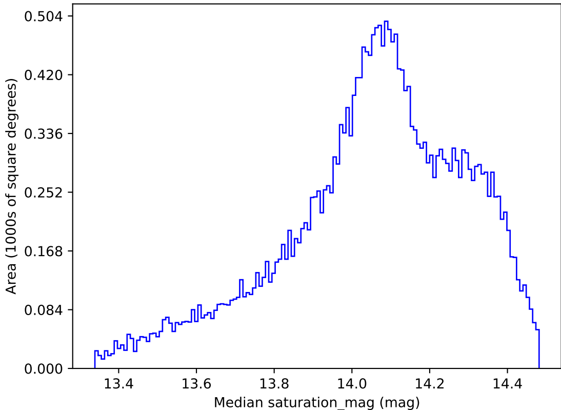
early_u_fpextra3.0_v3.4_10yrs All sky z band: Median saturation_mag
