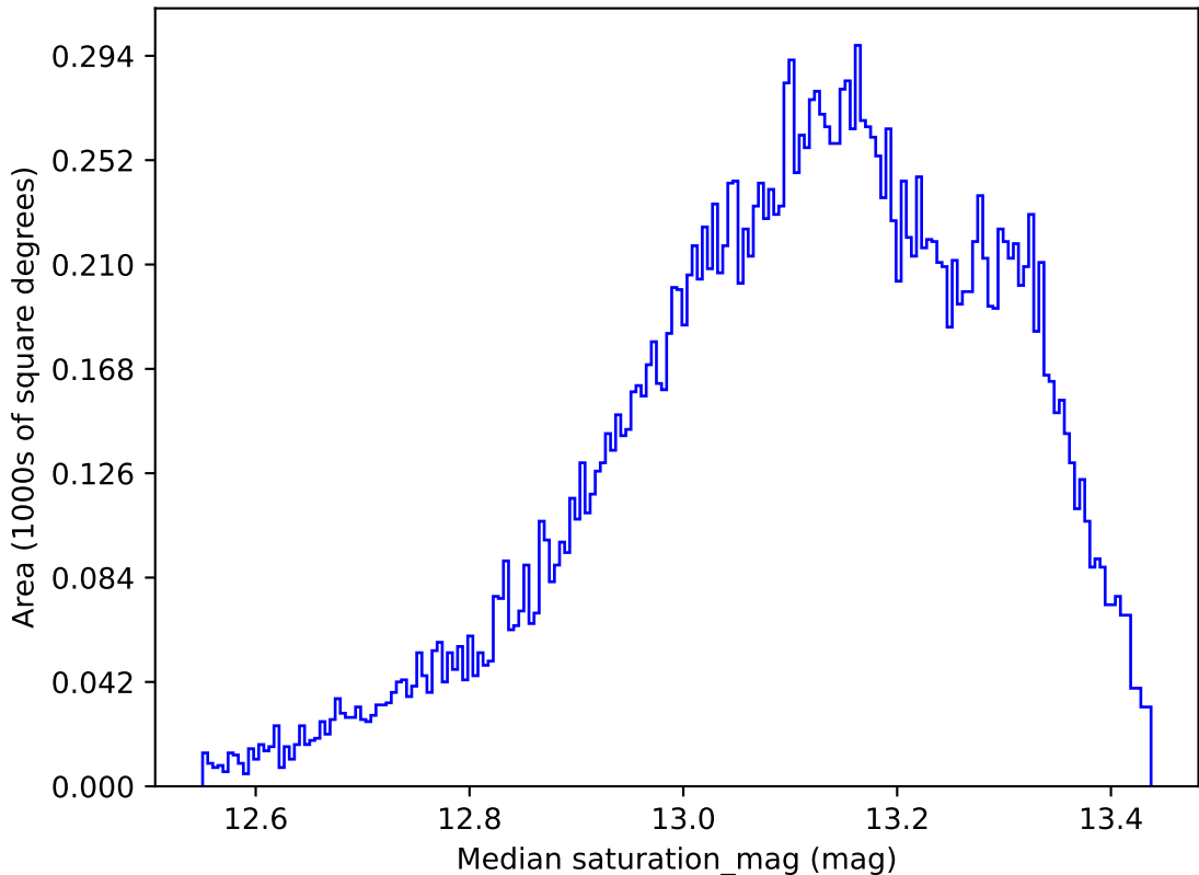
early_u_fpextra3.0_v3.4_10yrs All sky y band: Median saturation_mag
