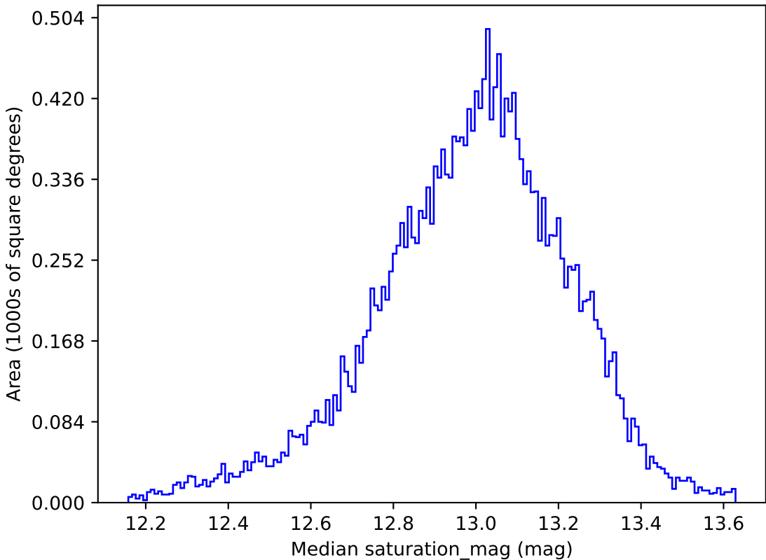
early_u_fpextra3.0_v3.4_10yrs All sky u band: Median saturation_mag
