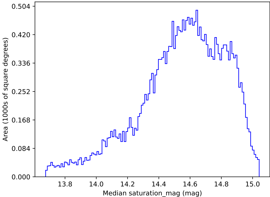
early_u_fpextra3.0_v3.4_10yrs All sky r band: Median saturation_mag
